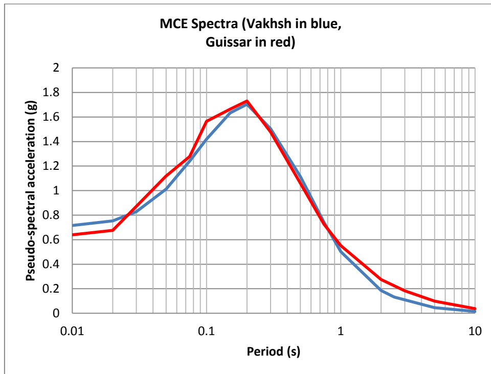
Figure 8: Comparison between the proposed response spectra for 5% damping associated to both the Guissar and Vakhsh faults.
