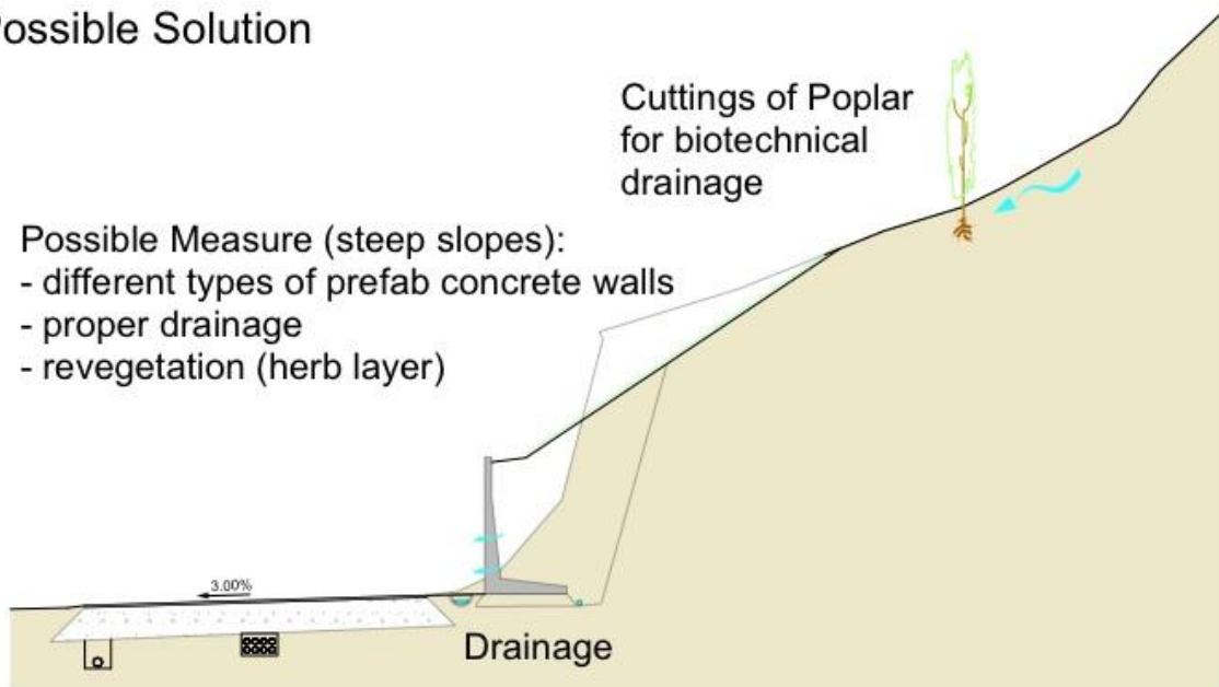
Figure 6: Slope stabilisation along roads
