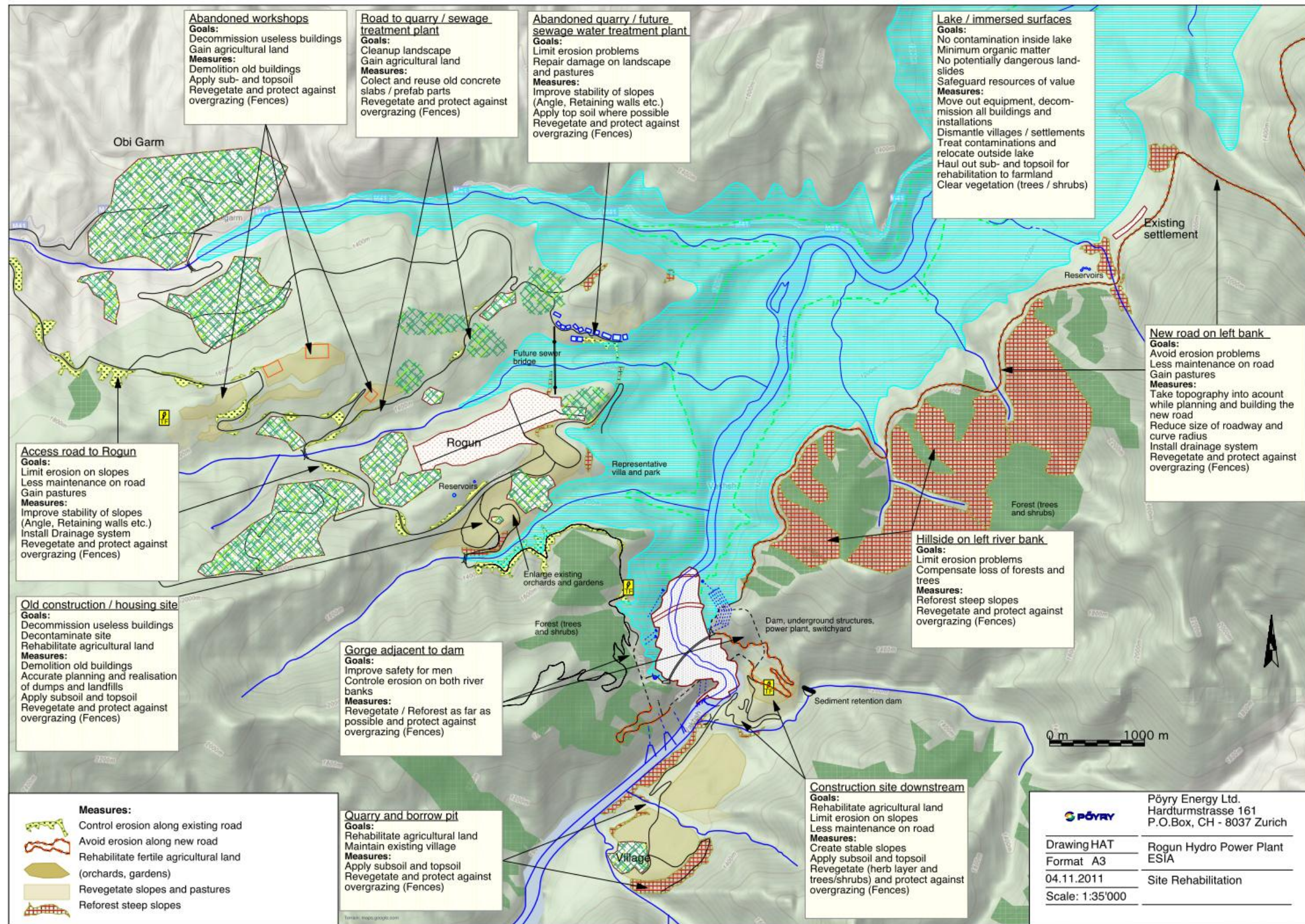
Figure 23: Rogun HPP: proposed site rehabilitation plan
