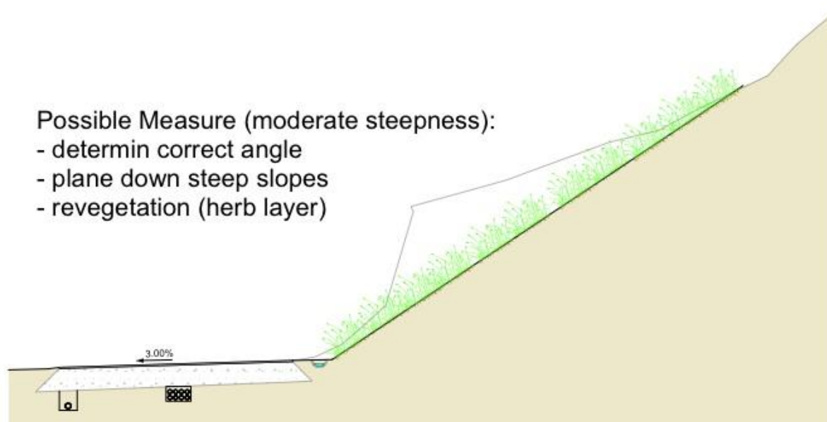
Figure 5: Simple way to get a stable slope with a layer of top soil and vegetation.
